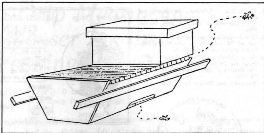
Top-bars from the KTBH are interchangeable into Langstroth boxes and the KTBH can be supered with Langstroth equipment. One or two top-bars removed from the end of the KTBH allow the bees access into the upper box. A few honey combs left in the KTBH at the end of the brood nest will discourage the queen from ascending into the super.
